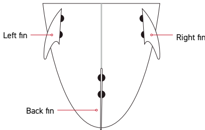
View from bottom of board at tail
